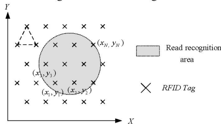
Fig. 9. RFID tag allocation and the recognition area of the reader in the triangular pattern.
