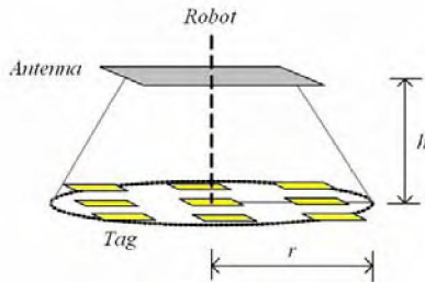
Fig. 2 Recognition area model of RFID antenna.
