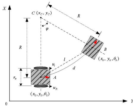
Fig. 12 Measurement and prediction model.
