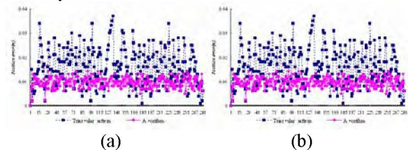
(a) Position error reduction. (b) Orientation error reduction. Fig. 17. Error reduction by the compensation algorithm.
